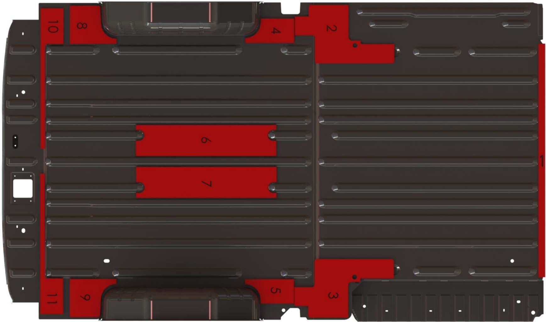
Layout of EVA Spacer Foam Revision 2
